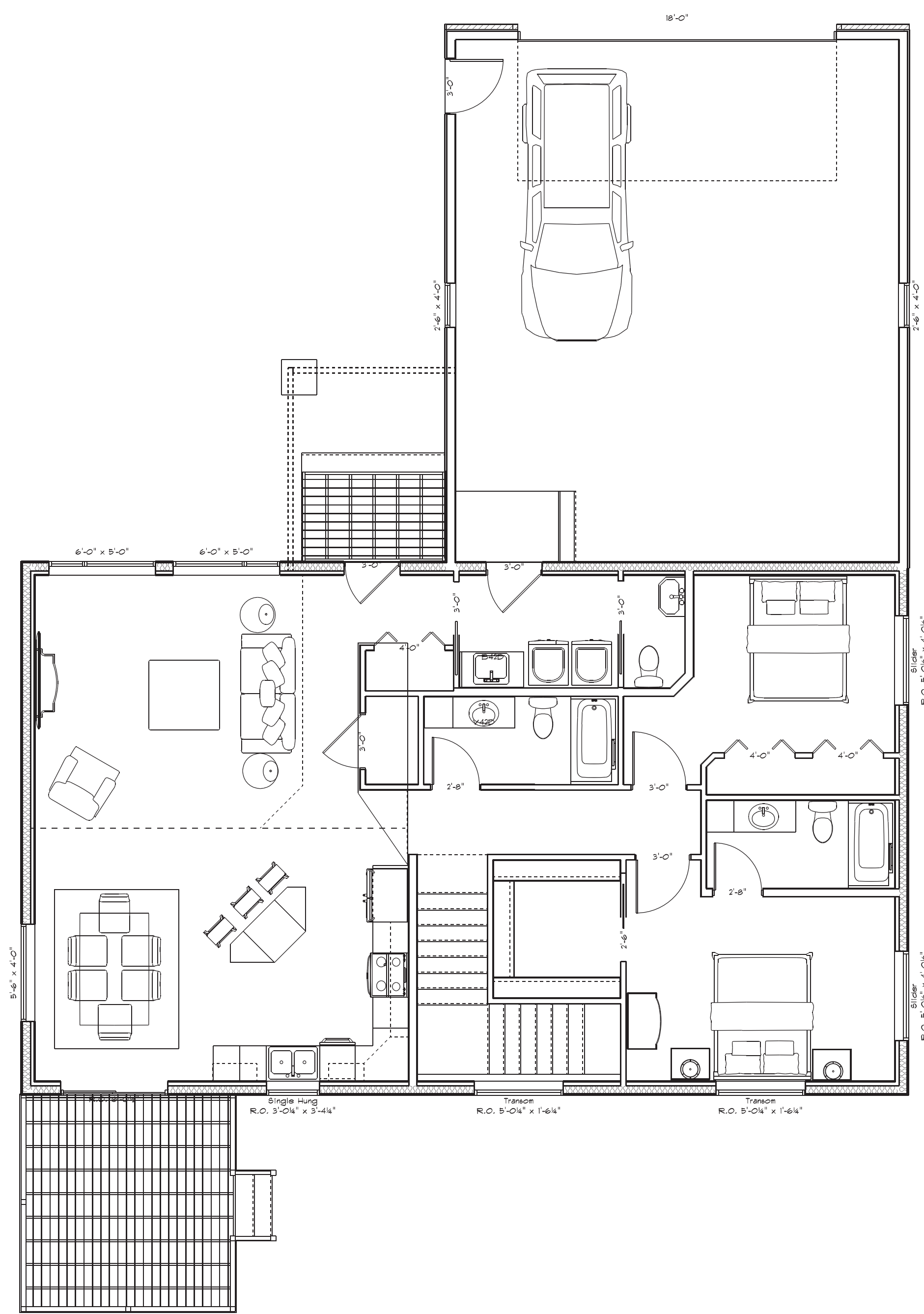
ProComm 1500 Floor Plan w Garage n Roof REV 8-5-2015
